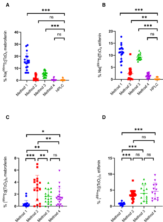
Figure 2 (A) Comparison of the percentage of \text{Na}^{99\text{m}}\text{Tc}(\text{TcO}_4) in ^{99\text{m}}\text{Tc} Tc-mefrofenin between Methods 1, 2, 3 and 4 and radio-high-performance liquid chromatography (radio-HPLC). Methods 5 and 6 use the same thin layer chromatography (TLC) characteristics as Method 4 for the search of \text{Na}^{99\text{m}}\text{Tc}(\text{TcO}_4) . A statistically significant difference was observed by the multiple comparison test between Method 1 and radio-HPLC ( p < 0.001 ) and between Method 3 and radio-HPLC ( p < 0.001 ). (B) Comparison of the percentage of \text{Na}^{99\text{m}}\text{Tc}(\text{TcO}_4) in ^{99\text{m}}\text{Tc} Tc-etifenin between Methods 1, 2, 3 and 4 and radio-HPLC. Methods 5 and 6 use the same TLC characteristics as Method 4 for the search of \text{Na}^{99\text{m}}\text{Tc}(\text{TcO}_4) . A statistically significant difference was observed by the multiple comparison test between Method 1 and radio-HPLC ( p < 0.001 ), between Method 2 and radio-HPLC ( p < 0.01 ) and between Method 3 and radio-HPLC ( p < 0.001 ). (C) Comparison of the percentage of ^{99\text{m}}\text{Tc}(\text{TcO}_2)_n in ^{99\text{m}}\text{Tc} Tc-mefrofenin between Methods 1, 2, 3 and 4. Method 5 uses the same TLC characteristics as Method 3, and Method 6 uses the same TLC characteristics as Method 1 for the search of ^{99\text{m}}\text{Tc}(\text{TcO}_2)_n . A statistically significant difference was observed by the multiple comparison test between Method 1 and Method 3 ( p < 0.01 ), and between Method 1 and Method 2 ( p < 0.001 ). (D) Comparison of the percentage of ^{99\text{m}}\text{Tc}(\text{TcO}_2)_n in ^{99\text{m}}\text{Tc} Tc-etifenin between Methods 1, 2, 3 and 4. Method 5 uses the same TLC characteristics as Method 3, and Method 6 uses the same TLC characteristics as Method 1 for the search of ^{99\text{m}}\text{Tc}(\text{TcO}_2)_n . A statistically significant difference was observed by the multiple comparison test between Methods 1 and 2 ( p < 0.001 ) and between Methods 1 and 3 ( p < 0.001 ). * p < 0.05 ; ** p < 0.01 ; *** p < 0.001 .
