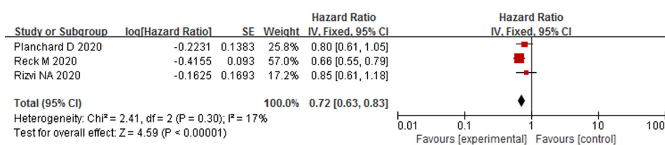
Figure 3 Forest plot of hazard ratios and 95% confidence intervals for overall survival of PD-1/PD-L1 plus CTLA-4 antibodies with lung cancer. CTLA-4, cytotoxic T lymphocyte antigen-4; PD-1, programmed cell death 1; PD-L1, programmed cell death-ligand 1.
