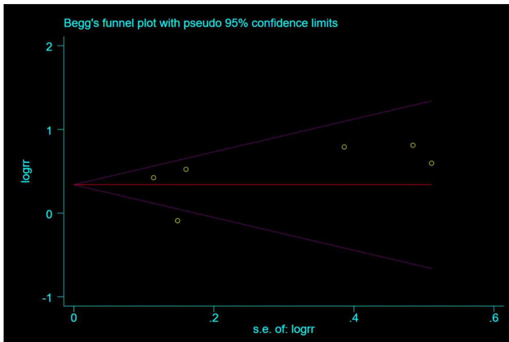
Supplemental figure 4 Begg's test of ratio risk on overall response rate.
